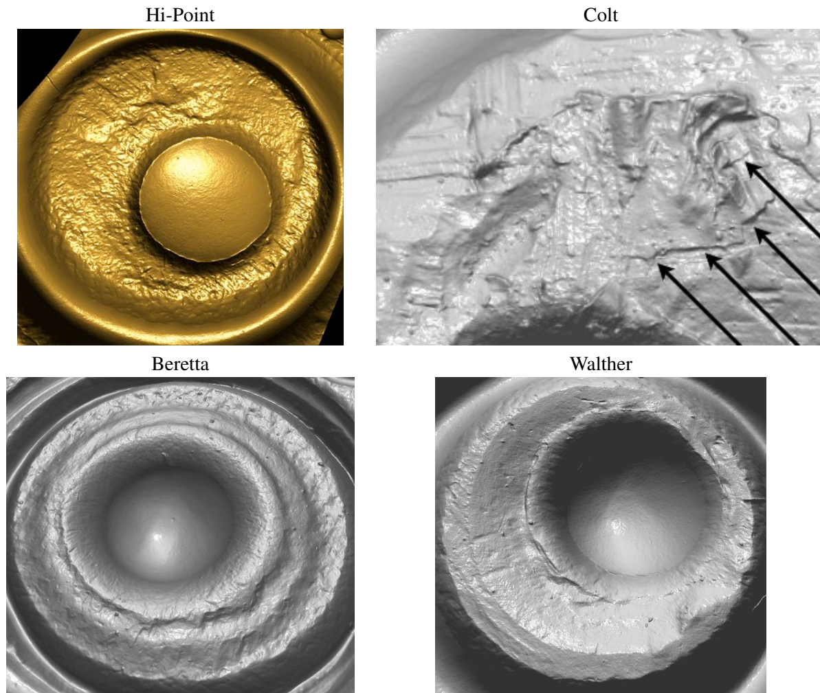
Figure 9: Examples of Difficult Scans. (Top-Left) Rendering (in brass color) of TopMatch-GS 3D scan of a Hi-Point (PMC brand ammunition) that was flagged as difficult to match by a firearms examiner but which was correctly matched using our algorithms. (Top-Right) Close-up of the ‘peeling’ effect seen in a number of RWS brand ammunitions. The edge of the peeling is highlighted with arrows. This represents an ammunition manufacturing defect confirmed by the manufacturer. (Bottom-Left) Rendering of a casing from a 9mm Beretta (Winchester brand ammunition) showing a very small region of breech-face impression. Despite the fact that most of the field-of-view is taken up by the flow-back our algorithm is able to correctly identify the known matching casing. (Bottom-Right) Rendering of a casing from a 9mm Walther (Remington brand ammunition) showing a poorly-marked and sloped breech-face impression. The scarcity of features on this casing prevented a match from being found. The top two casings were included in the 47-firearm experiment, all four were included in the Large Data Set Test.
