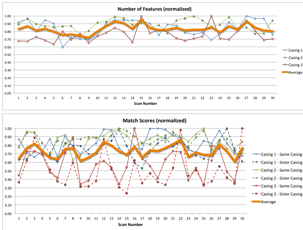
Figure 12: Replicate Studies. (Top) The Number of features detected on each replicate scan for the three test casings. The number of features are normalized so that the maximum number of features for each casing have a value of 1.0. The average (thick orange line) shows that there is no downward trend. The number of detected features is fairly consistent over time. (Bottom) The Match scores for each of the three casings to a second scan of itself (Same Casing, solid line) and to a different, sister, casing from the same firearm (Sister Casing, dashed line). The scores for each of the six experiments are normalized so that the largest score for each experiment has a value of 1.0. The average (thick orange line) shows that the average match scores do not decrease with repeat scans.
