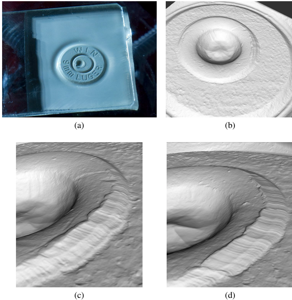
Figure 2: Sensor and Sample Images. (a) An image of a 9mm Luger cartridge case breech-face pressed into the elastomeric sensor. The surface topography of the breech-face is captured using our method, based on [10]. (b) The rendering of a captured surface. (c) and (d) Closeups of the surface topography of two different cartridge cases that were fired through the same firearm. The images show both primer shear marks and breech-face impressions. Note that although the proposed work is not yet addressing the automated comparison of primer shear marks, the the two images reliably capture the similarity between the two tool marks. Note that images were downsampled for presentation. In the original images, a single pixel corresponds to 1.7 microns. In the results described below, images are captured at 1.4 microns per pixel. The system has a maximum resolution of 0.8 microns per pixel.
