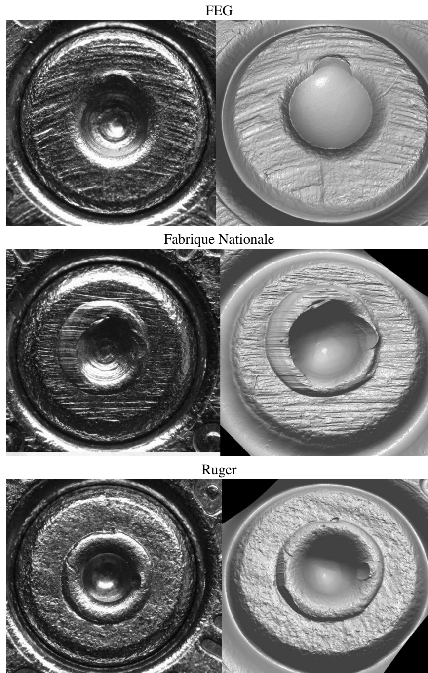
Figure 8: Three Examples of Good Scans. Three scans using the PMC brand ammunition (brass case, brass primer). In each pair, a traditional light microscope image is shown on the left while a rendering of the TopMatch-GS 3D collected surface is shown on the right. All three casings match correctly. (Top) FEG brand firearm showing milled marks. (Middle) Fabrique Nationale brand firearm showing filed type marks. (Bottom) Ruger brand firearm showing granular impressed marks.
