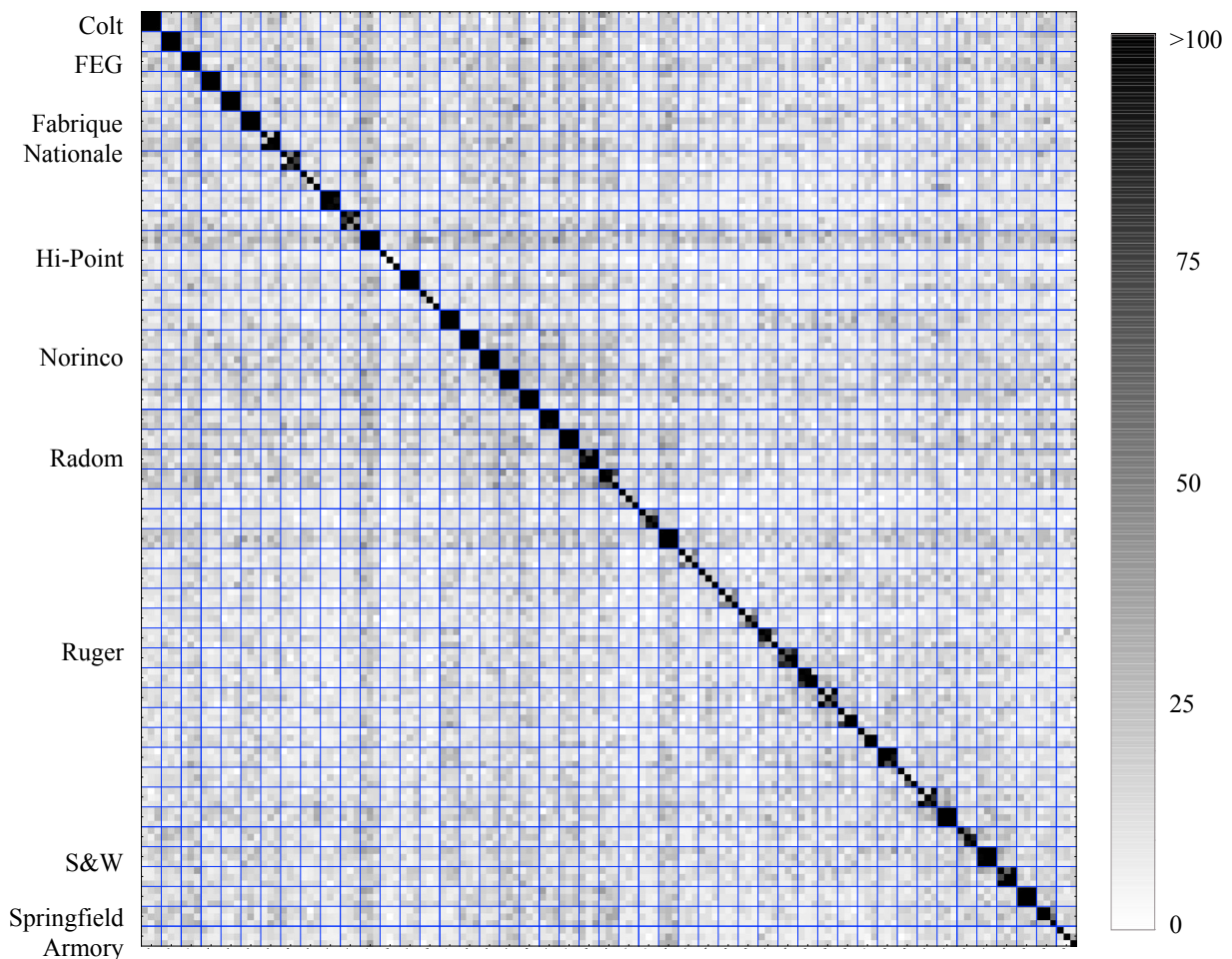
Figure 10: Experiment One (47 Firearms, 141 Cases) Confusion Matrix. The result of 19,881 comparisons. Each cell in the matrix corresponds to the match score between two casings (specified by the involved row and column). The firearms are grouped by manufacturer and separated in the matrix by thick blue lines. Match scores go from white (indicating a score of zero) to black (indicating a score of at least 100). The three test fires from each firearm are presented in order. Thus we expect a series of small 3x3 boxes of correct matches along the diagonal of this graph (each 3x3 box captures the match scores of the 3 test fires from each firearm with themselves, i.e. , correct matches). Most firearms match extremely well, with a small tight black 3x3 patch of known matches. The KNM are in the ‘off-diagonal’ position, they are all white or very light grey indicating a small match score. A clearer view of a similar confusion matrix appears in Figure 11.
