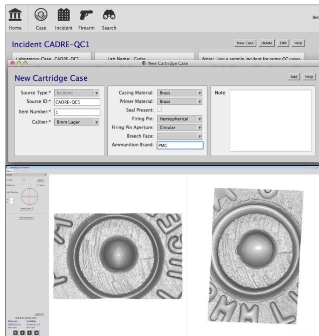
Figure 6: User Interface Software Images. Our prototype user interface software allows the firearms examiner the ability to visualize, database, search, and score casings. (Top) Example window showing the primary object types ( i.e. , Casings, Incidents, and Firearms) and data entry for the creation of a new Casing. (Bottom) Example side-by-side 3D visualization of two matching casings. These two casings have a high match score and have been automatically identified and aligned by our software. The user can lock the two casings such that they rotate together and can rotate the casings both in the plane and in full 3D.
