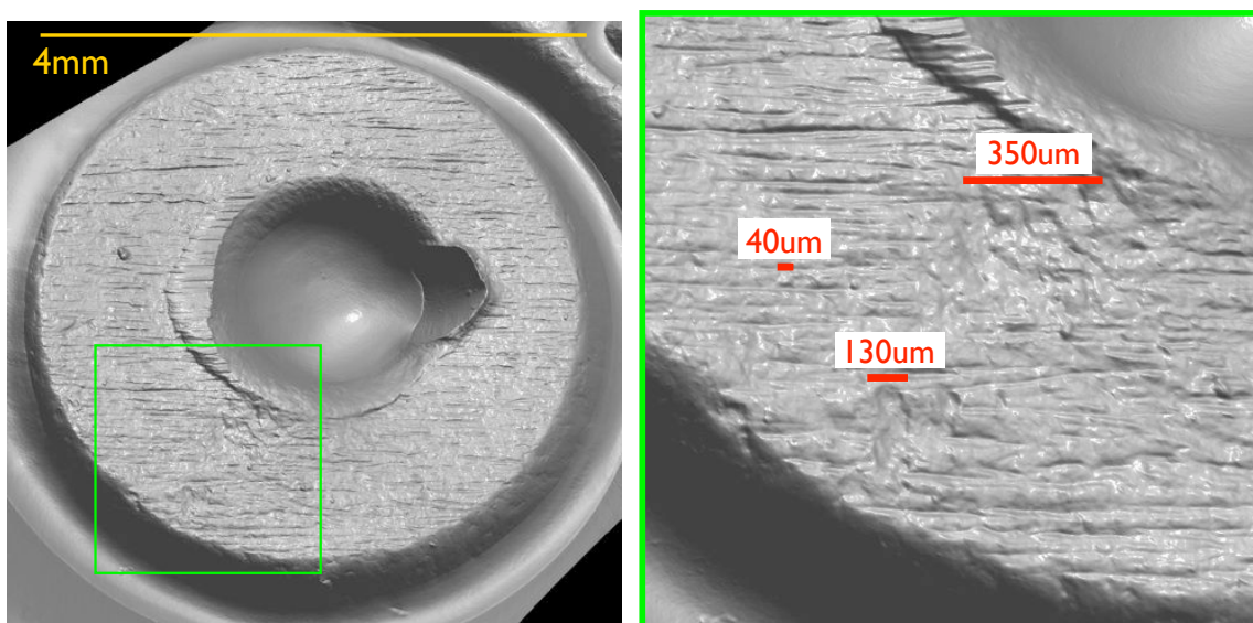
Figure 1: Feature Sizes. A 3D scan of the NIST Standard Casing illustrating several distinct features with their approximate sizes. (Left) The NIST standard casing. (Right) a close-up of the boxed region of the left image. Firearms examiners often rely on features 10\mu\text{m} and larger.
