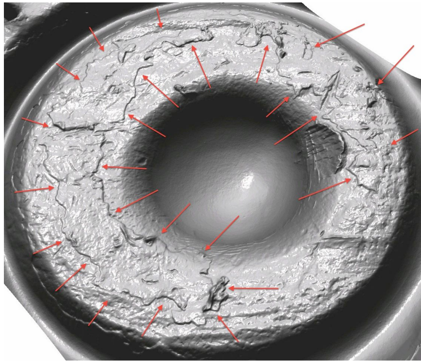
Figure 7: Winchester Ammunition with Lacquer. A rendered view of the 3D measured surface of a primer that had been covered with a protective lacquer prior to firing. The lacquer can be seen as a skin which lies on the surface of the primer and bunches in some locations (see arrows). The lacquer can obstruct the tool mark transfer process. In this example, the identifiable features of the breech-face impression have not transferred and the casing is not identifiable with sister casings from the same firearm.
