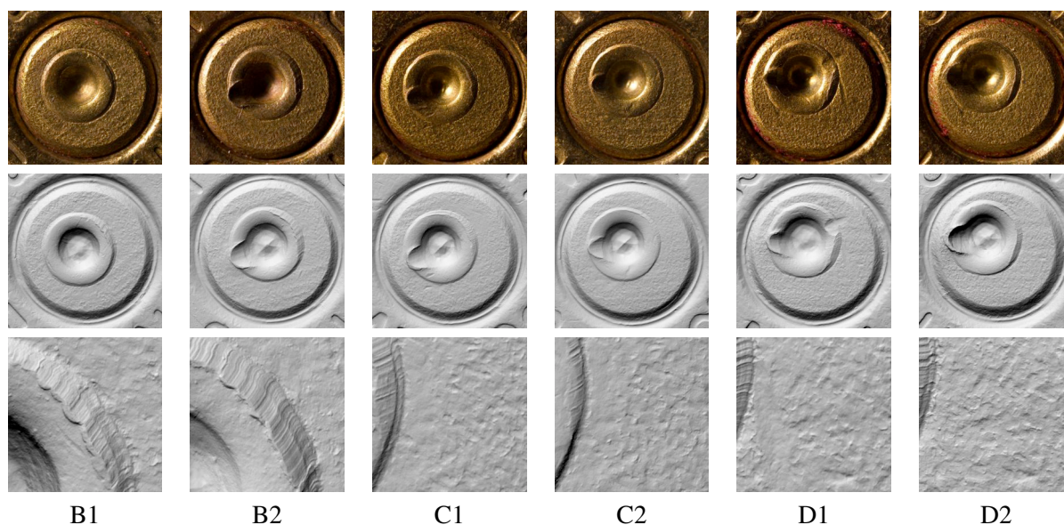
Figure 4: Case Scans. Six cartridge cases, two from each of three firearms (denoted B, C, and D). (Top) Traditional light microscope color images of the six cartridge cases. (Middle) Renderings of the measured geometry of each casing. (Bottom) Close-up view from each scan showing the detail that can be measured using our system. Note that these images are not at full resolution. The actual scans capture features beyond 2 micron resolution.
