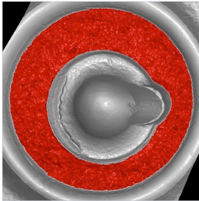
Figure 5: Breech-Face Impression Mask. The auto-masked region containing the breech-face impression is shown in red. Note that the firing pin impression, primer shear, and ejector marks are not included in the current matching algorithm. In most cases, the mask identified by the auto-masker can be used directly, on occasion the user will want to manually touch-up the mask around the edges.
